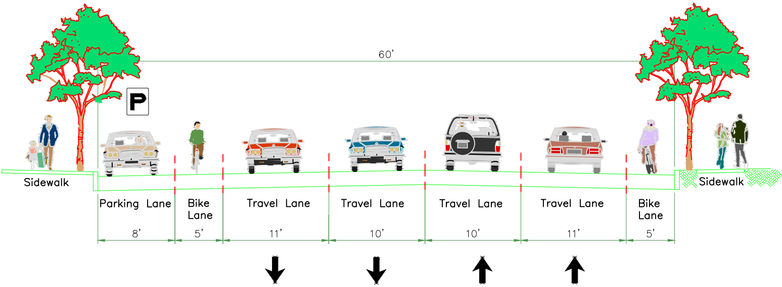
PROPOSED MADISON ROAD SECTION LOOKING WEST
