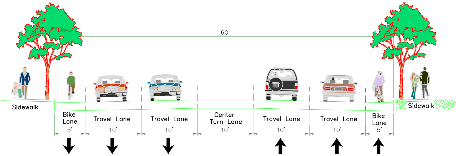
PROPOSED MADISON ROAD SECTION LOOKING WEST
