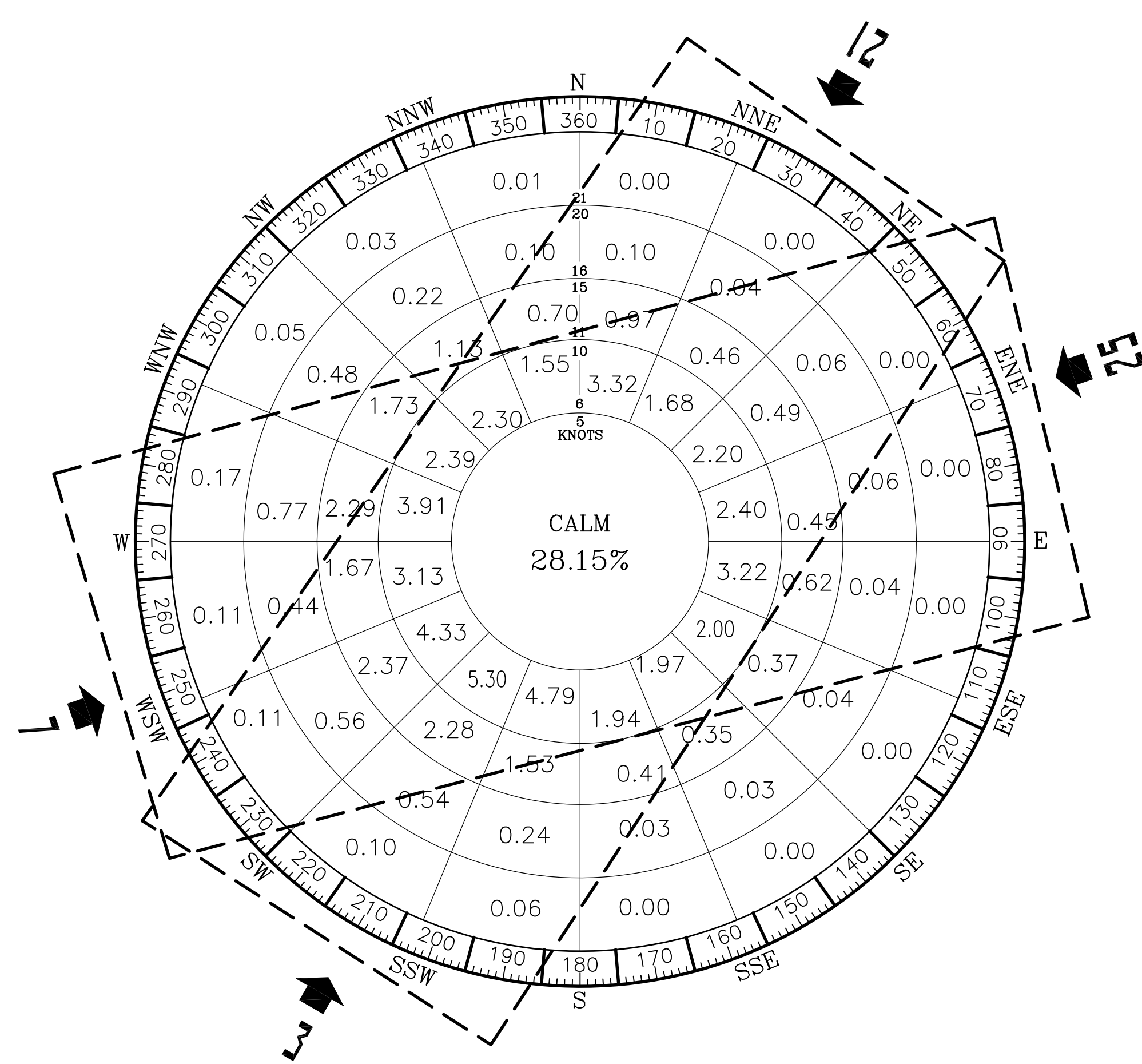
ALL WEATHER WIND ROSE
