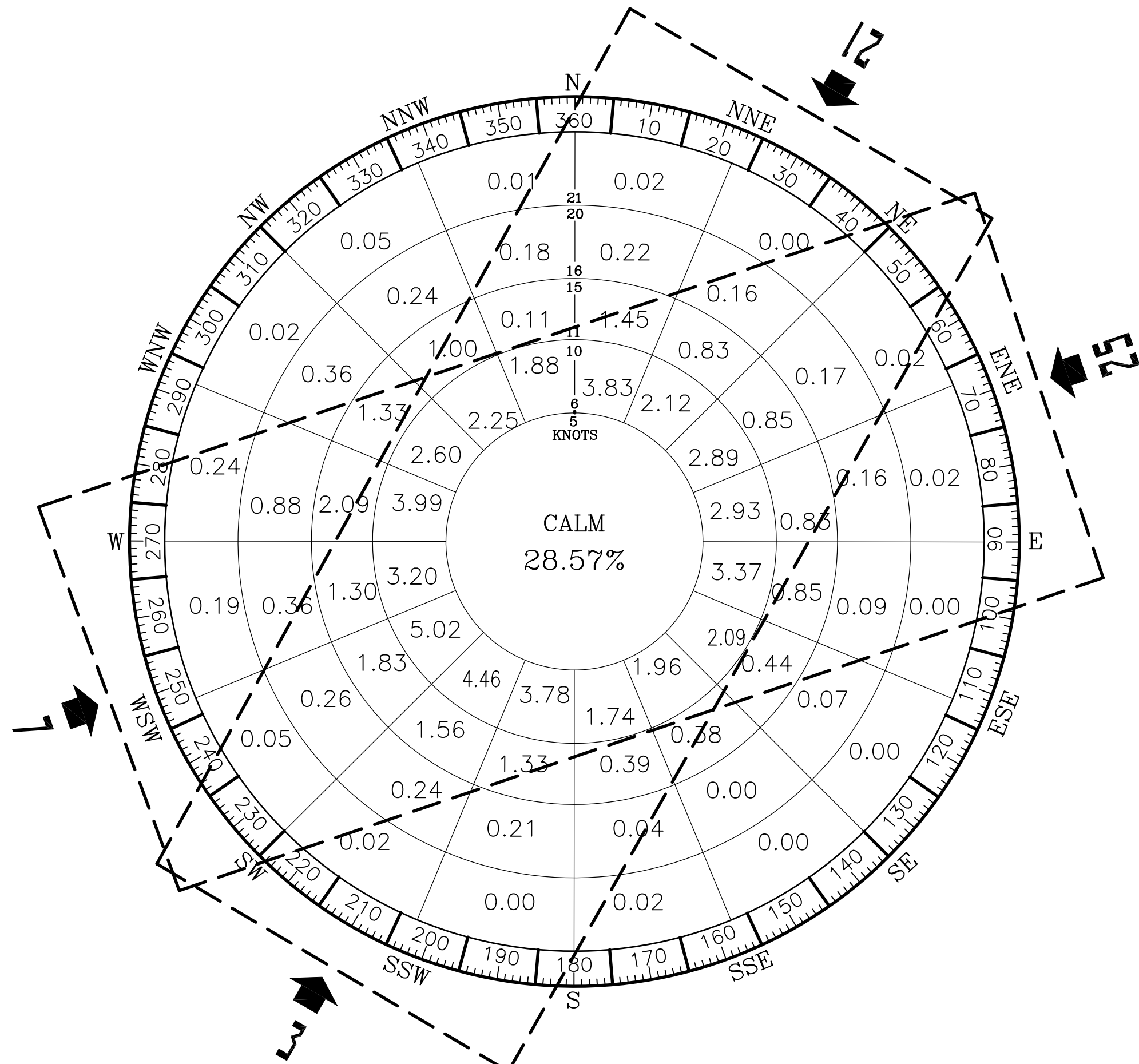
IFR WIND ROSE
