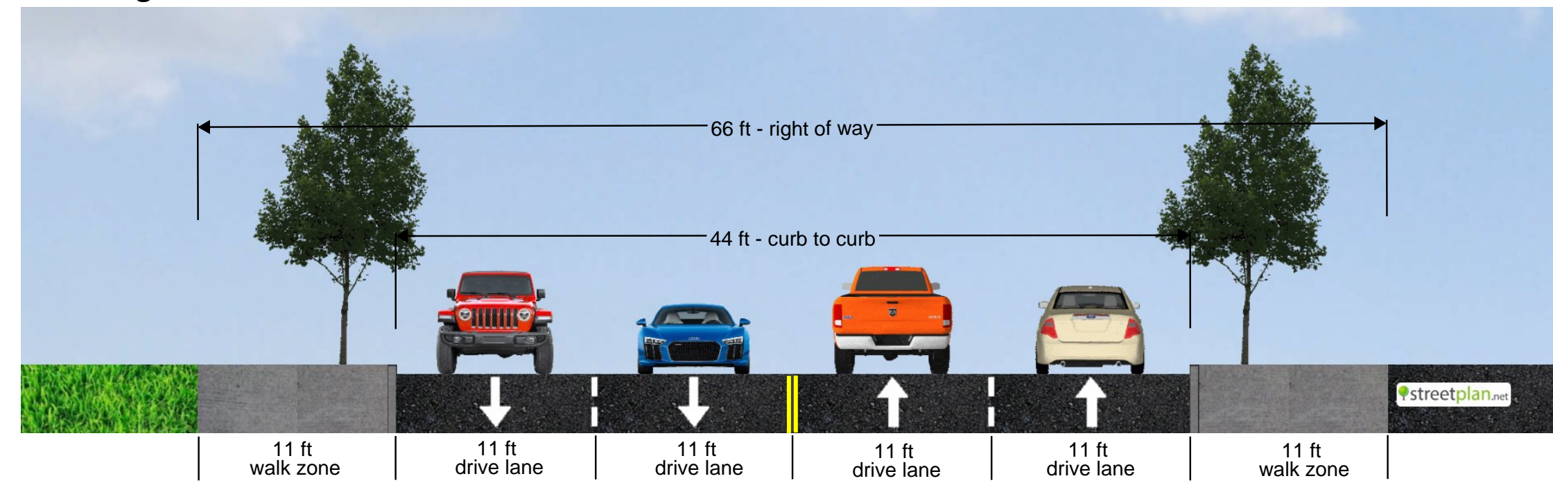
Court Street Roadway Section
