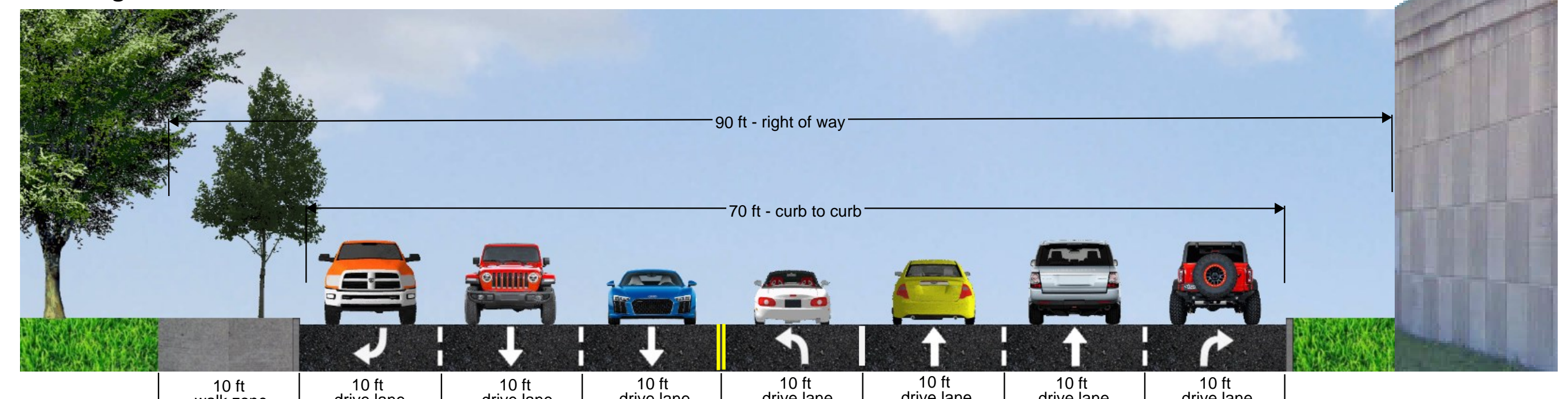
Gilbert Ave - Court to Casino Roadway Section
